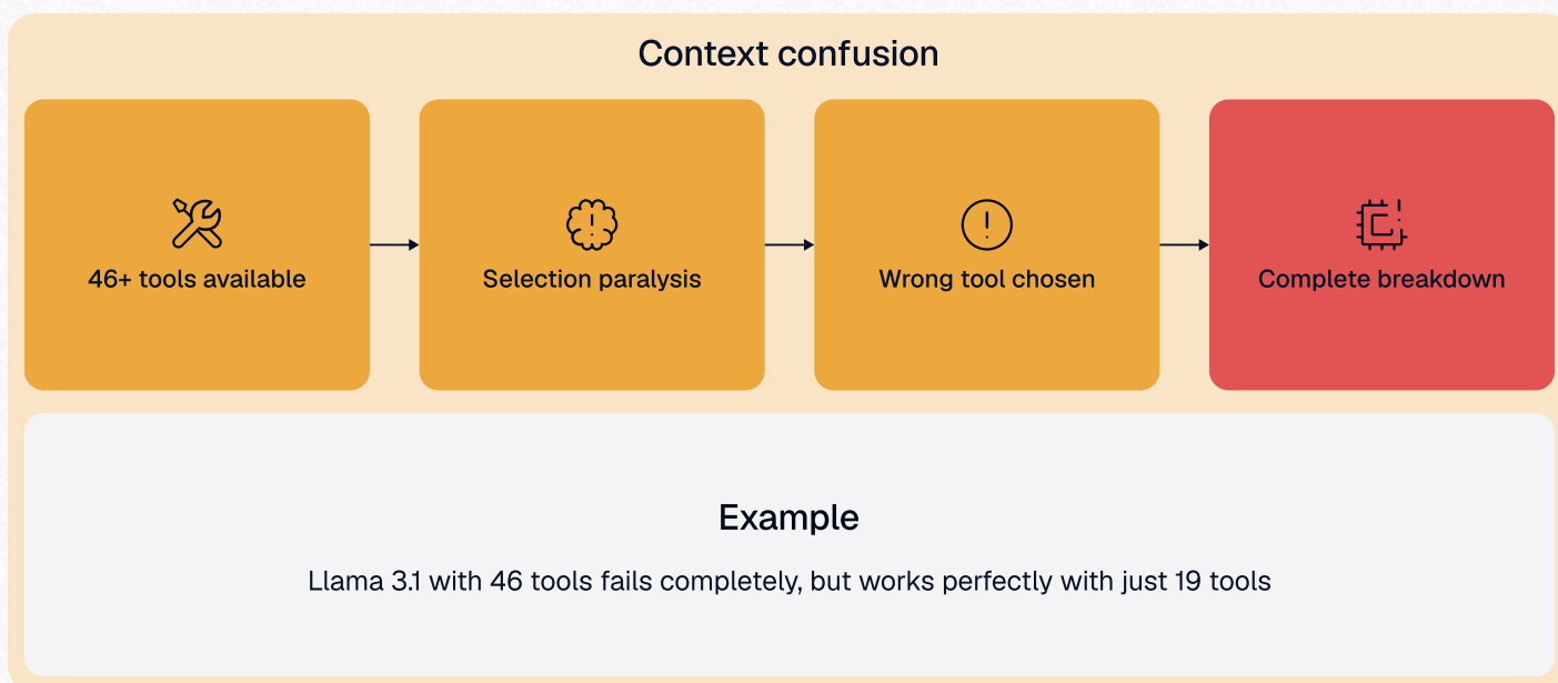
FIGURE 4.4 Context confusion from tool overload to complete breakdown
