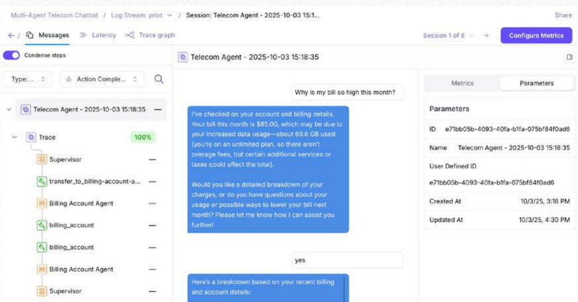
FIGURE 5.4 Action Completion step
